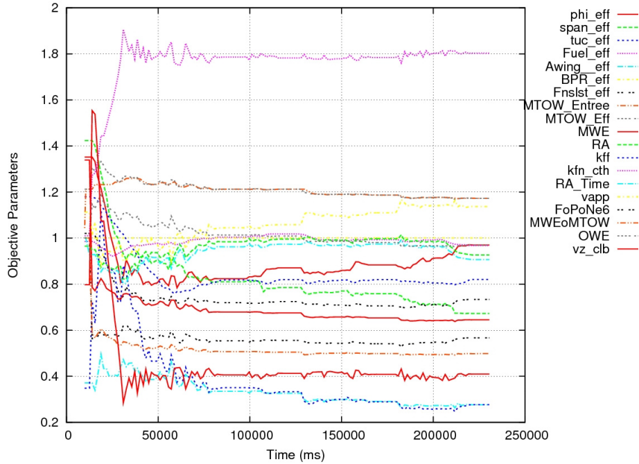
Figure 6: Evolution of objective parameters during a Mascode execution
