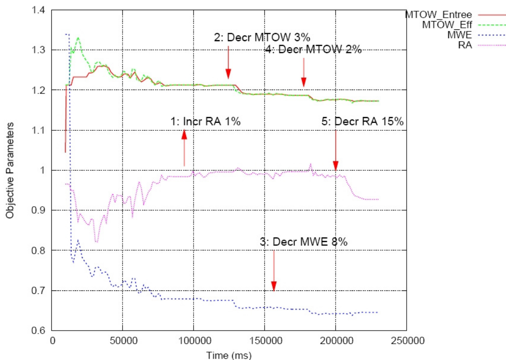
Figure 8: Values of parameters RA , MTOW and MWE
