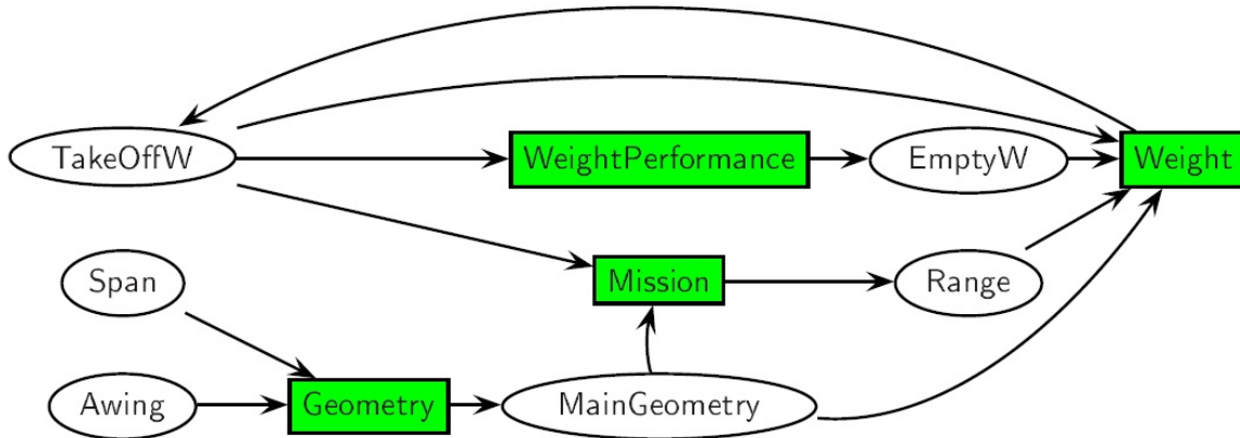
Figure 1: A simplified example of relation between models
