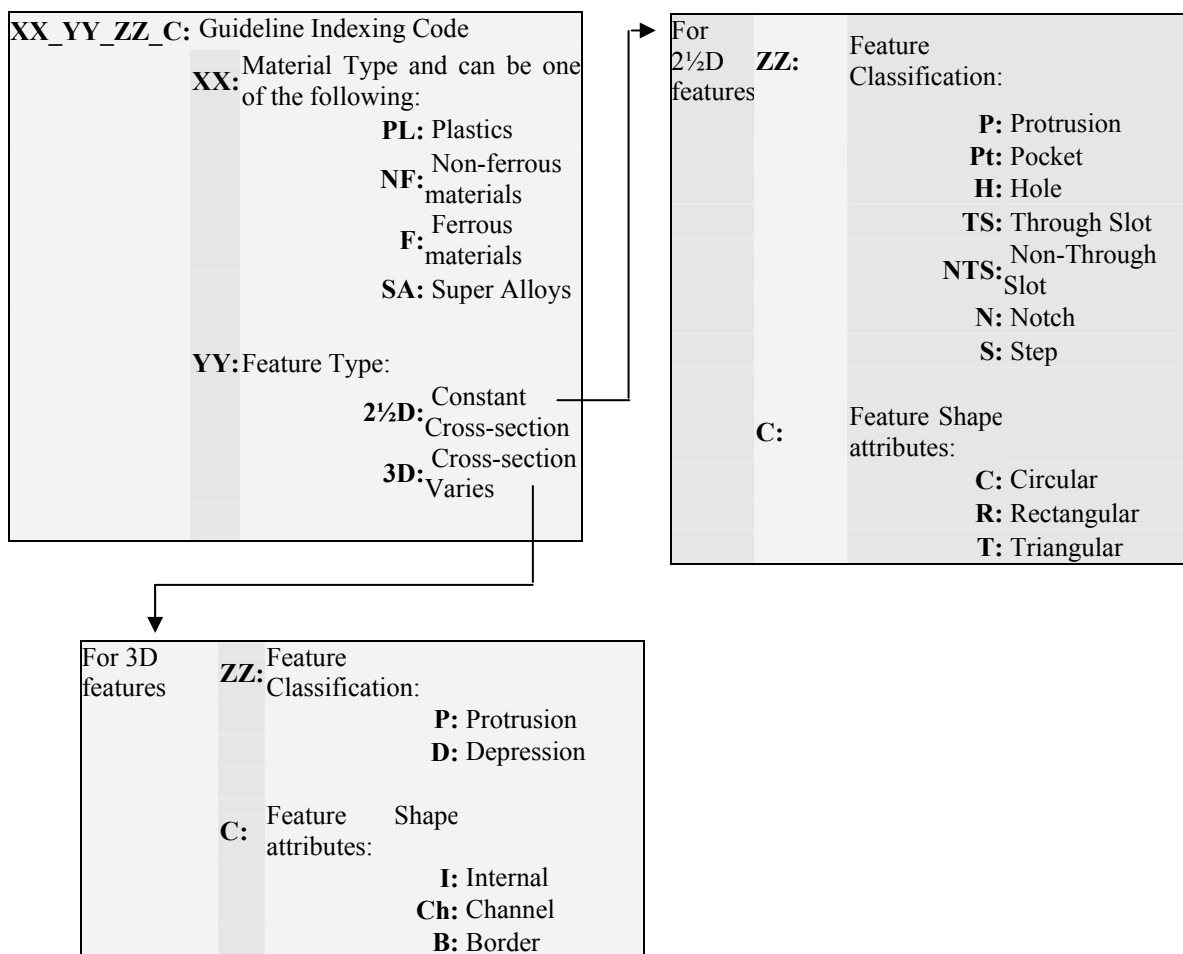
Figure 4. Guideline Indexing
